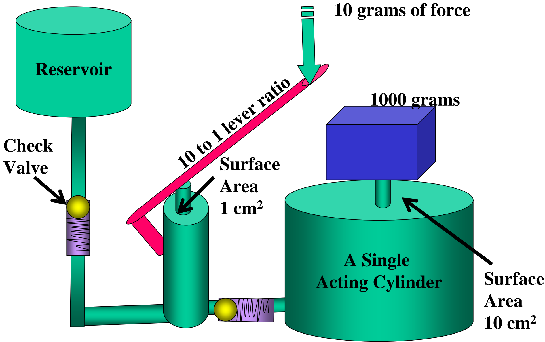
A Hydraulic Jack System
